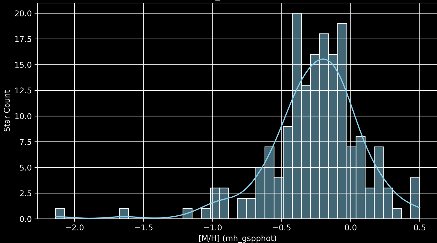
APOGEE DR17 Field: [115-48_MGA [M/H] (mh_gspphot) (n= 174)
