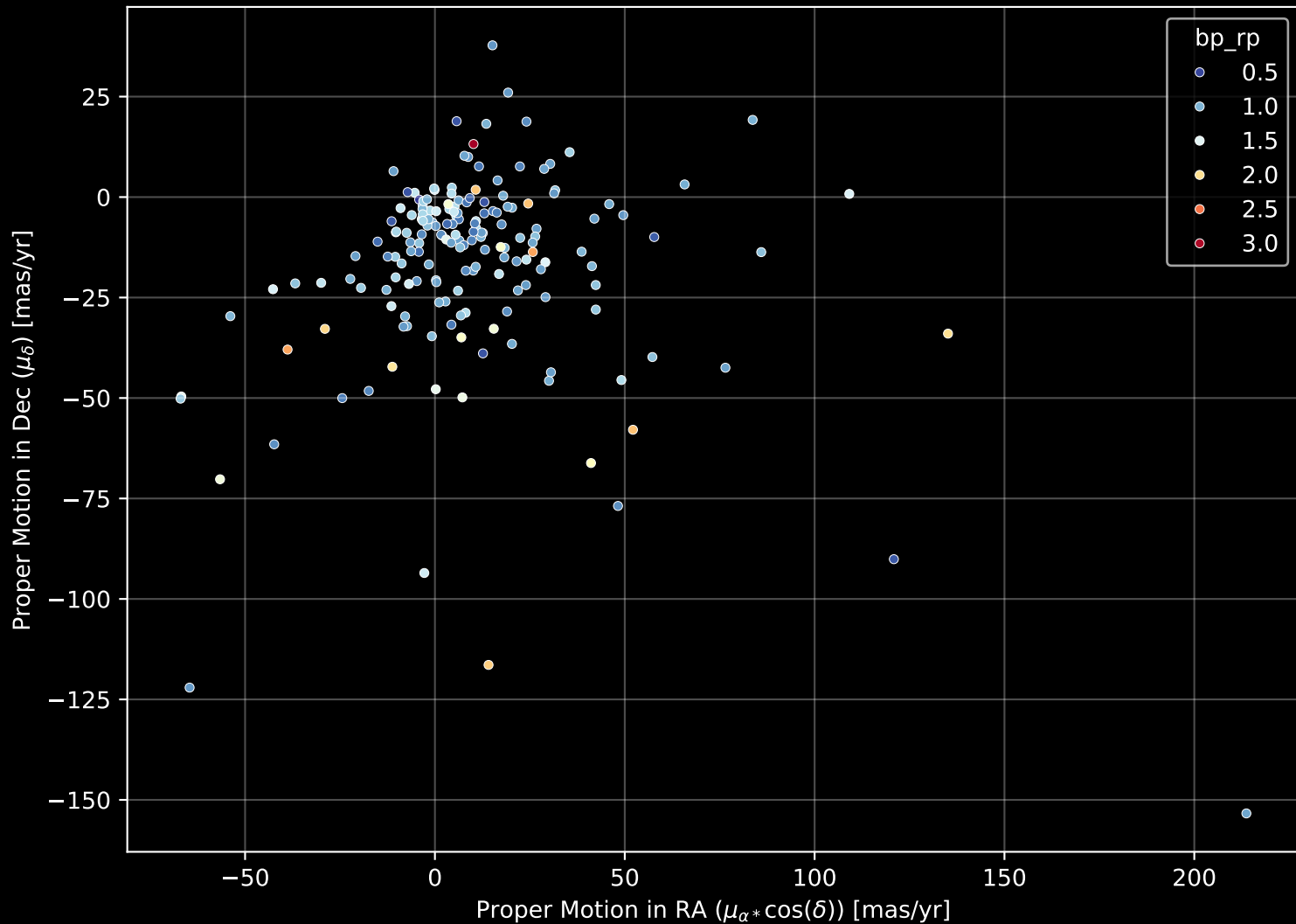
APOGEE DR17 Field: [115-48_MGA] Proper Motion Diagram (n= 177)
