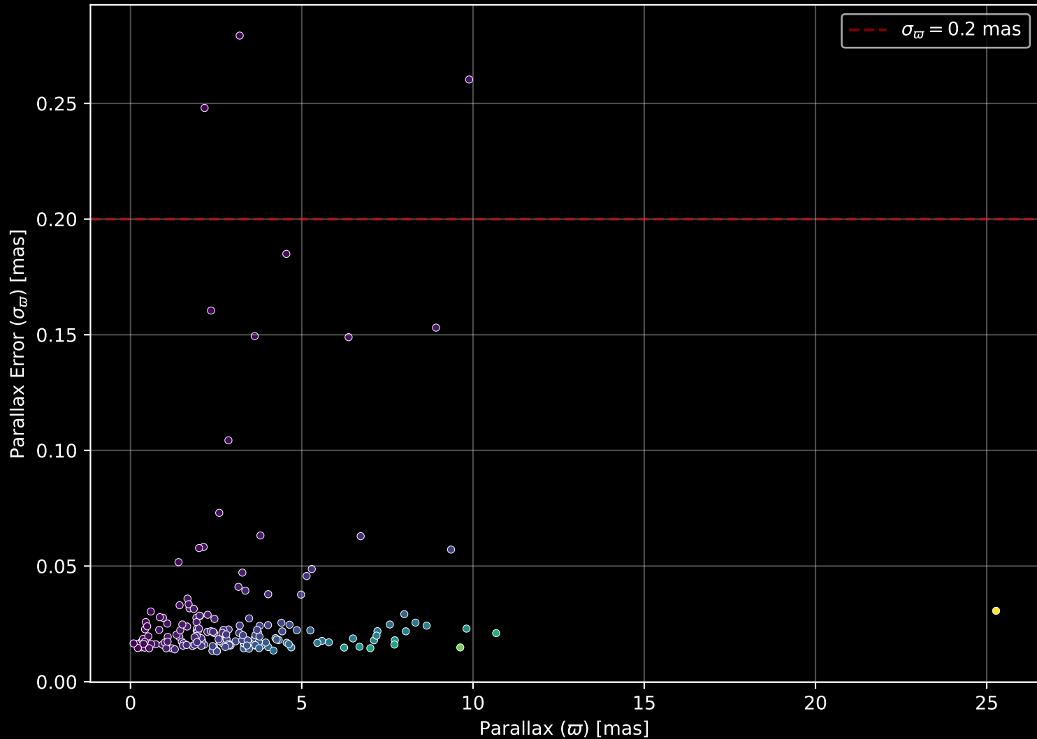
APOGEE DR17 Field: [115-48_MGA] Parallax Quality (n= 177)
