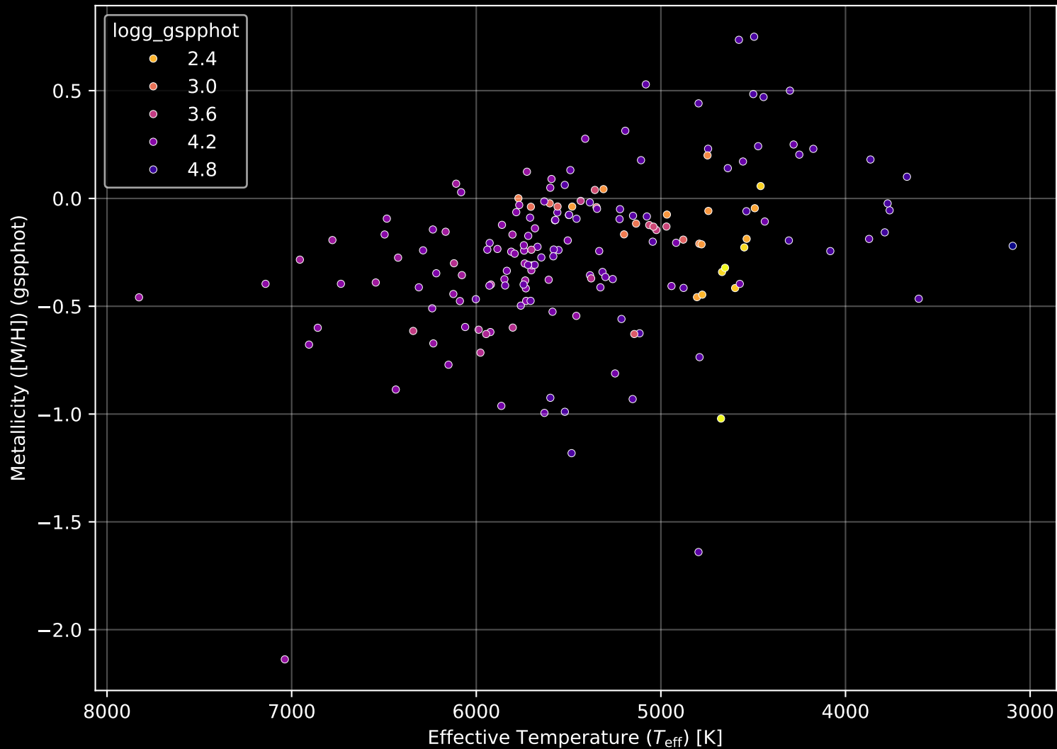
APOGEE DR17 Field: [115-48_MGA] Stellar Population Parameters (n= 177)
