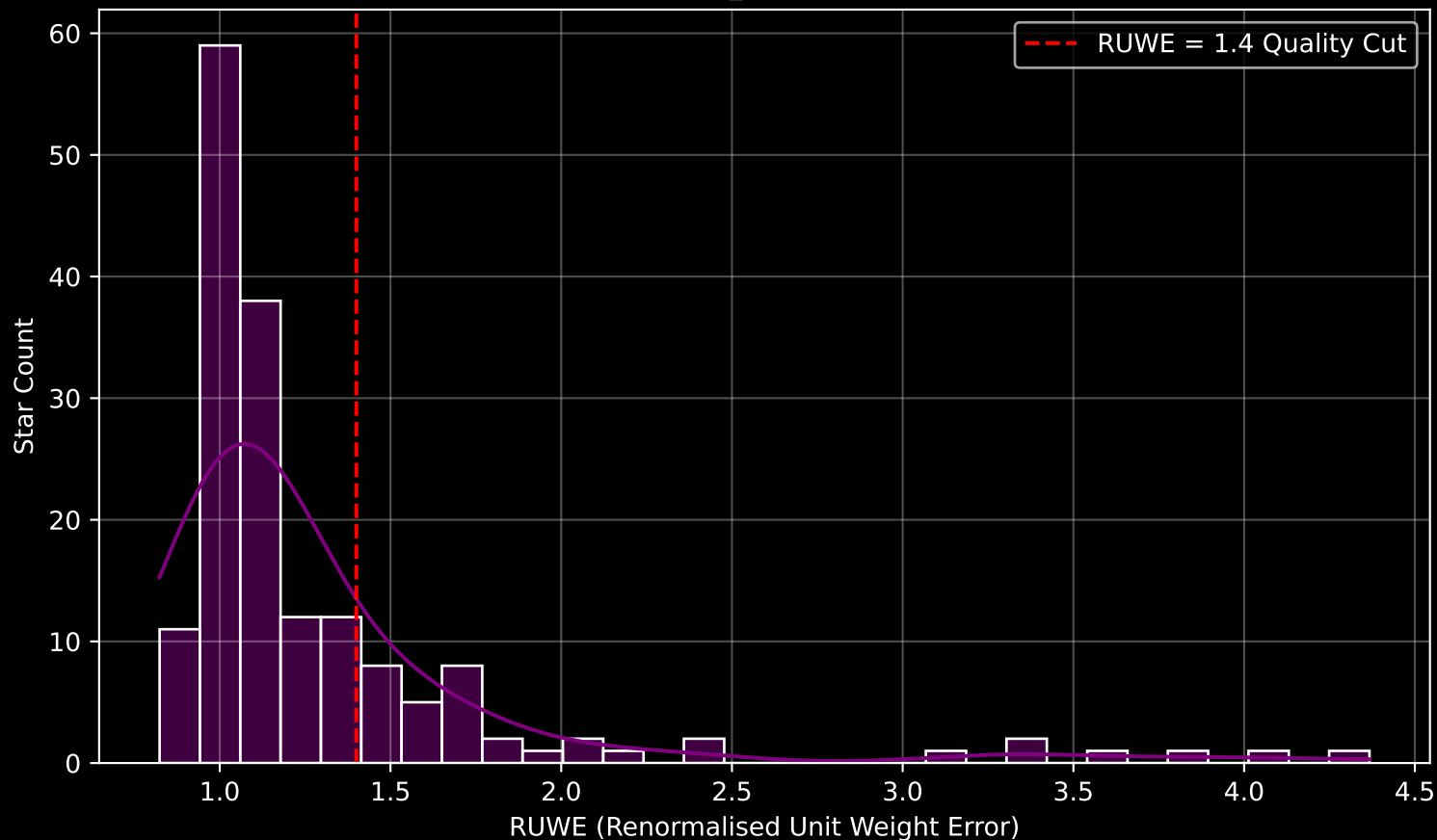
GAPOGEE DR17 Field [115-48_MGA] RUWE Distribution (n= 168)
