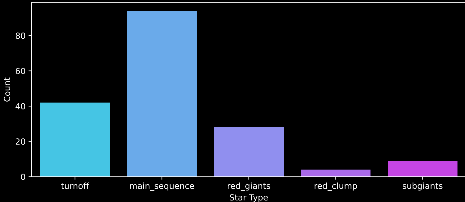
APOGEE DR17 Field: [115-48_MGA] Count plot of Star Type
