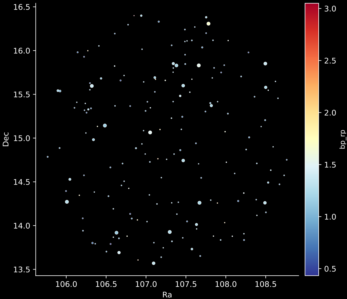
APOGEE DR17 Field: [115-48_MGA] Stars: 177
